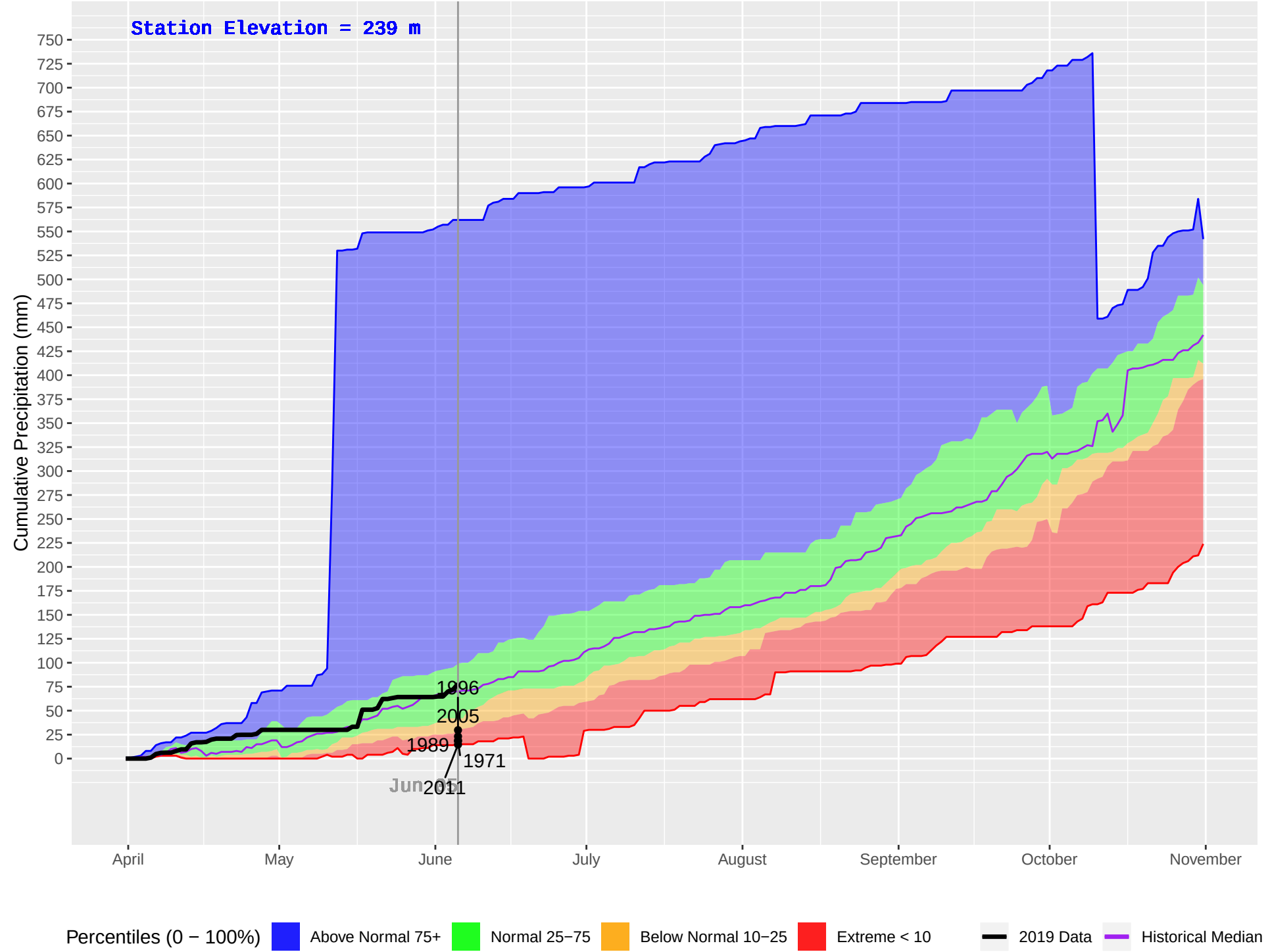
ROSSWOOD (105) : Historical (1970–2018), Current (2019) Daily Cumulative Precipitation
