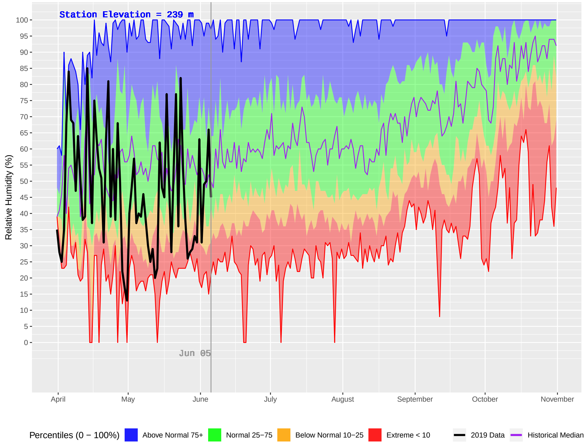
ROSSWOOD (105) : Historical (1970–2018) and Current (2019) Daily Relative Humidity
