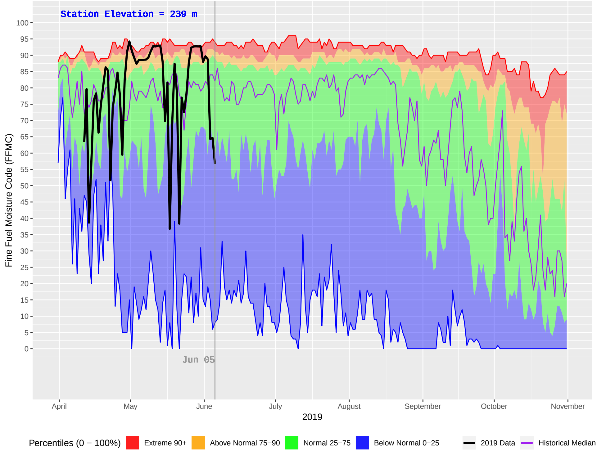
ROSSWOOD (105) : Historical (1970–2018) and Current (2019) Daily Fine Fuel Moisture Code (FFMC)
