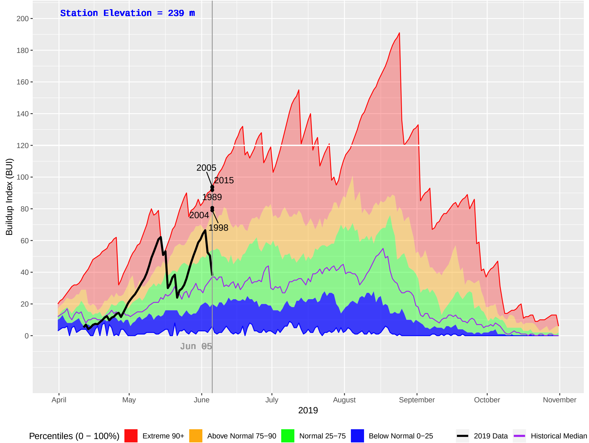
ROSSWOOD (105) : Historical (1970–2018), Current (2019) Daily Buildup Index (BUI)
