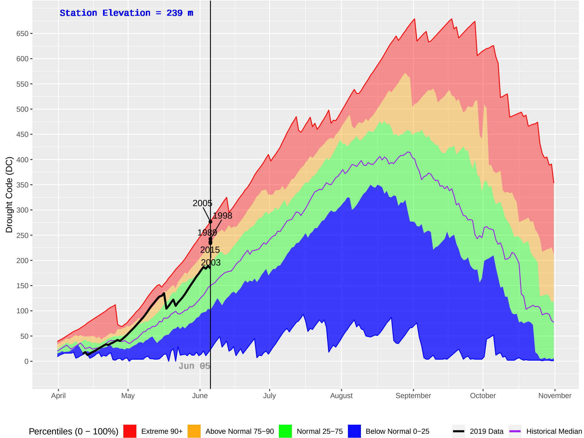
ROSSWOOD (105) : Historical (1970–2018) and Current (2019) Daily Drought Code (DC)
