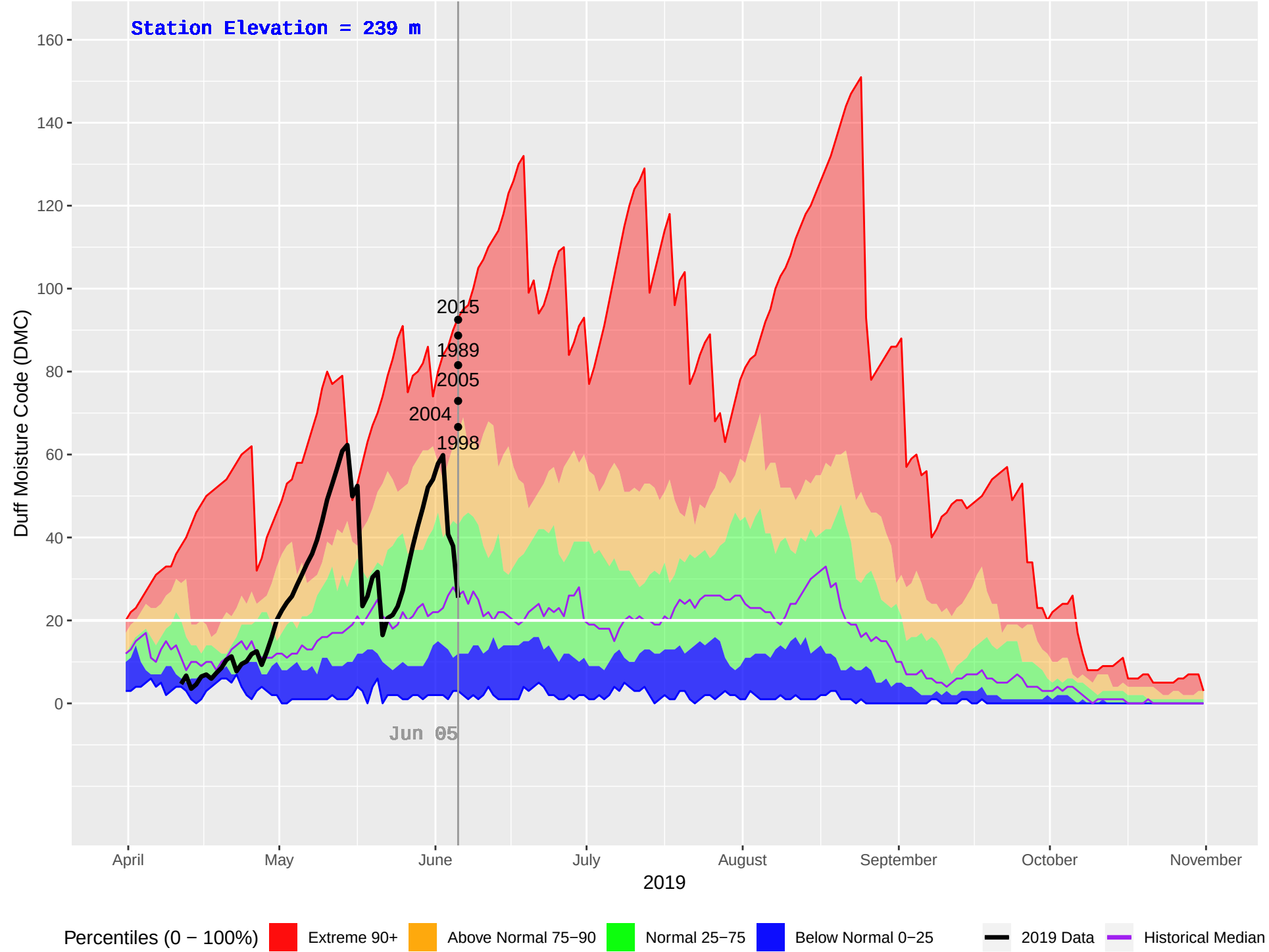
ROSSWOOD (105) : Historical (1970–2018), Current (2019) Daily Duff Moisture Code (DMC)
